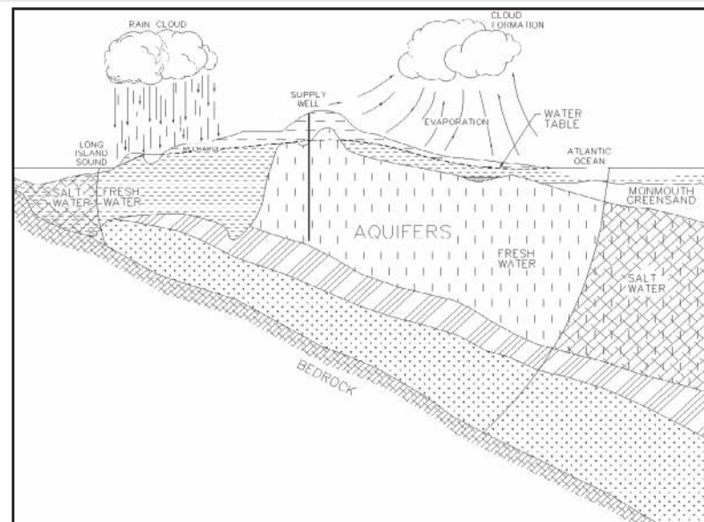
THE LONG ISLAND AQUIFER SYSTEM
